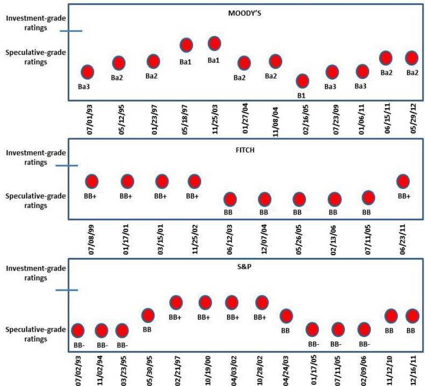
Figure 1. CRAs Credit Rating for the Philippines, 1993-2011
